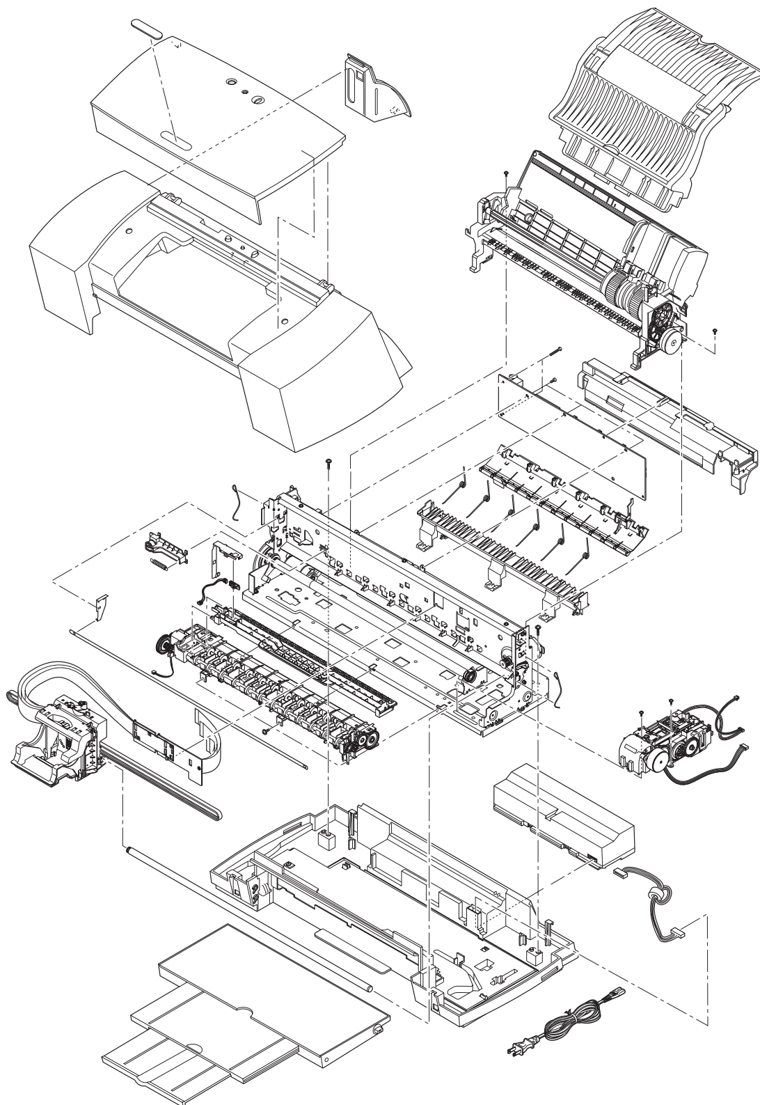
Figure 2-3 Exploded View
