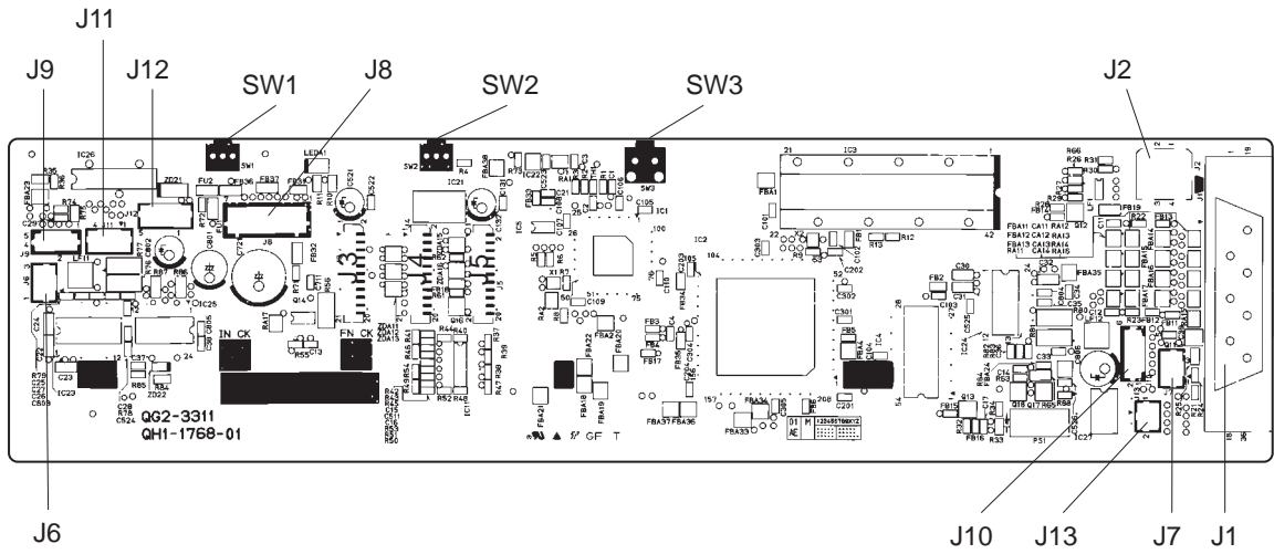
Figure 4-1 Control Board
