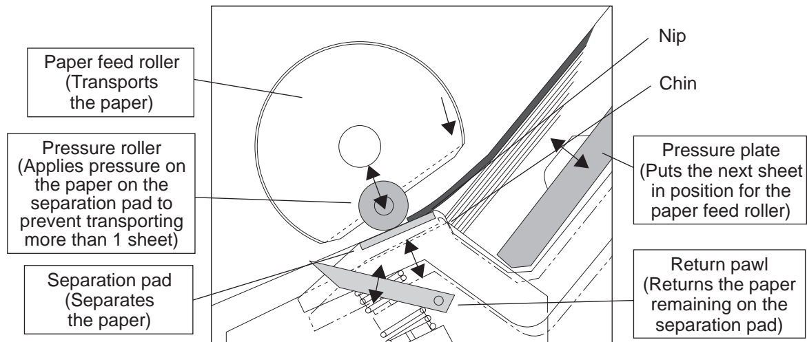
Figure 3-11 Paper Feeding
